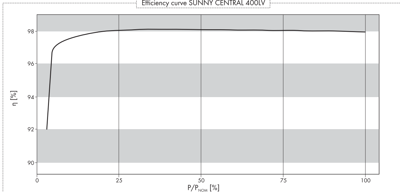
Efficiency curve SUNNY CENTRAL 400LV
